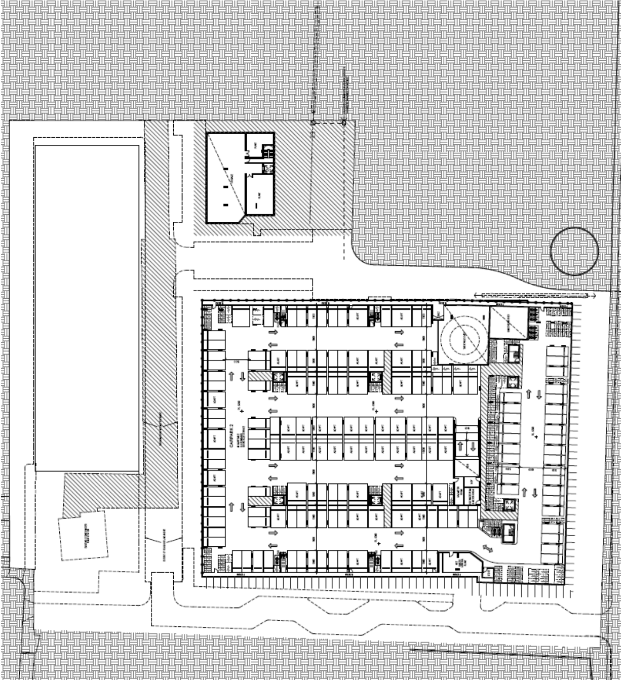
Basement Plan
