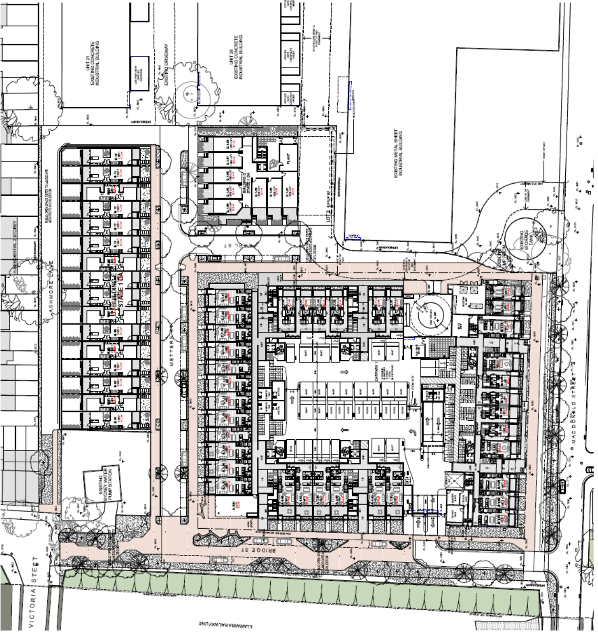
Level 1 (Ground) Floor Plan
